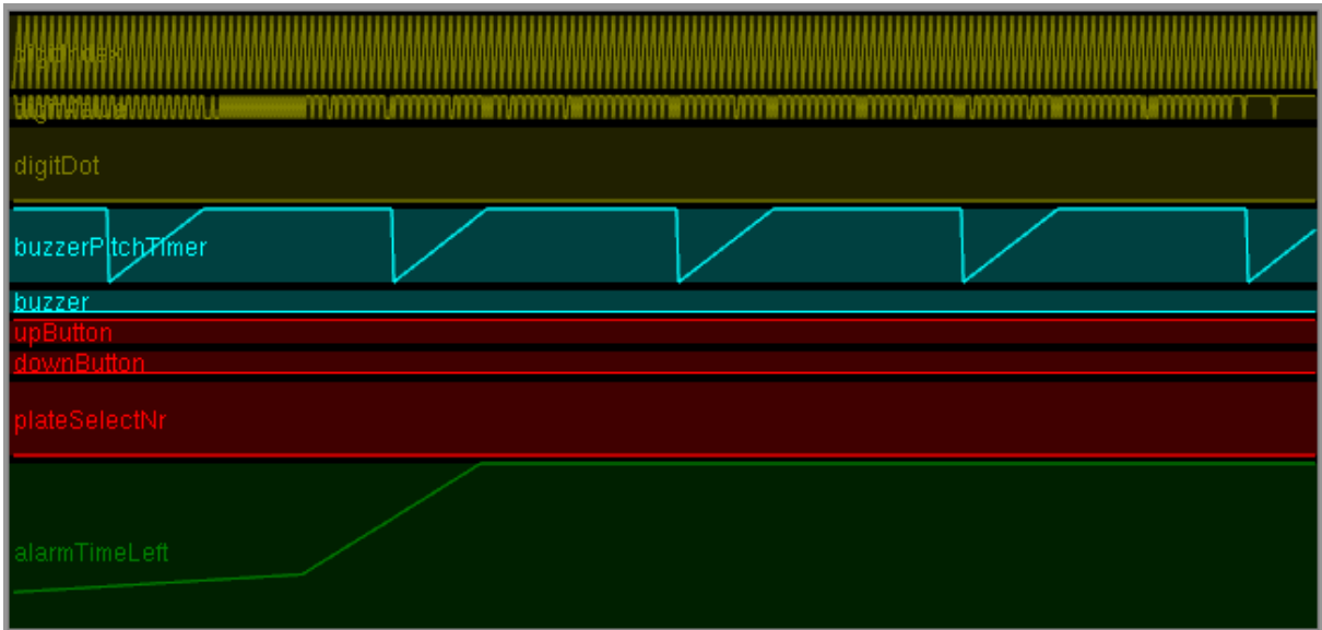
Figure 8. Timing chart of the stove example.
