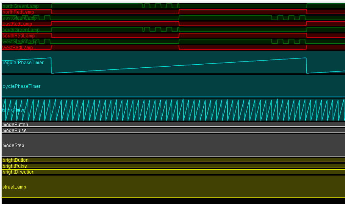
Figure 2. Timing chart of the traffic light example in regular mode.
